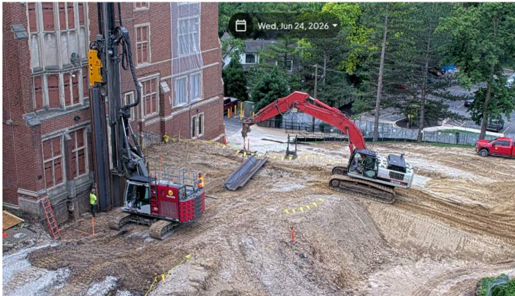
Earth Retention System Installation Process
